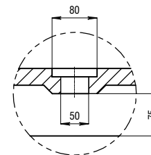
DETAIL D SCALE 1:3
