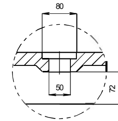
DETAIL D SCALE 1:3
