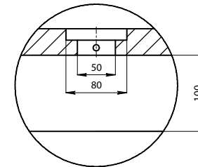
DETAIL D SCALE 1:4
